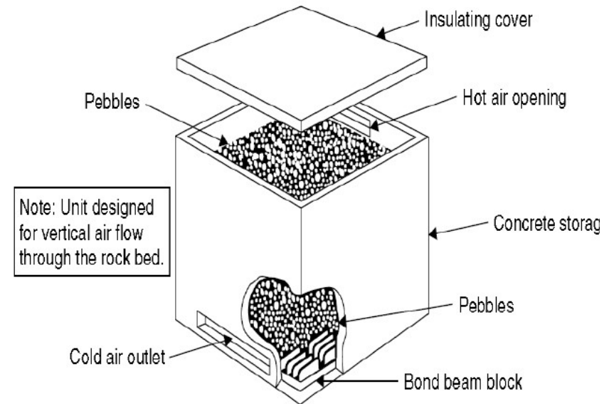
Vertical flow packed rock bed.
