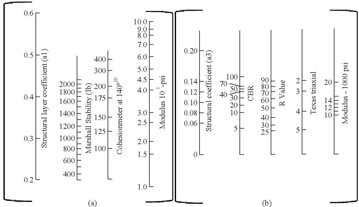
Variation in (a1) with surface course strength parameters
