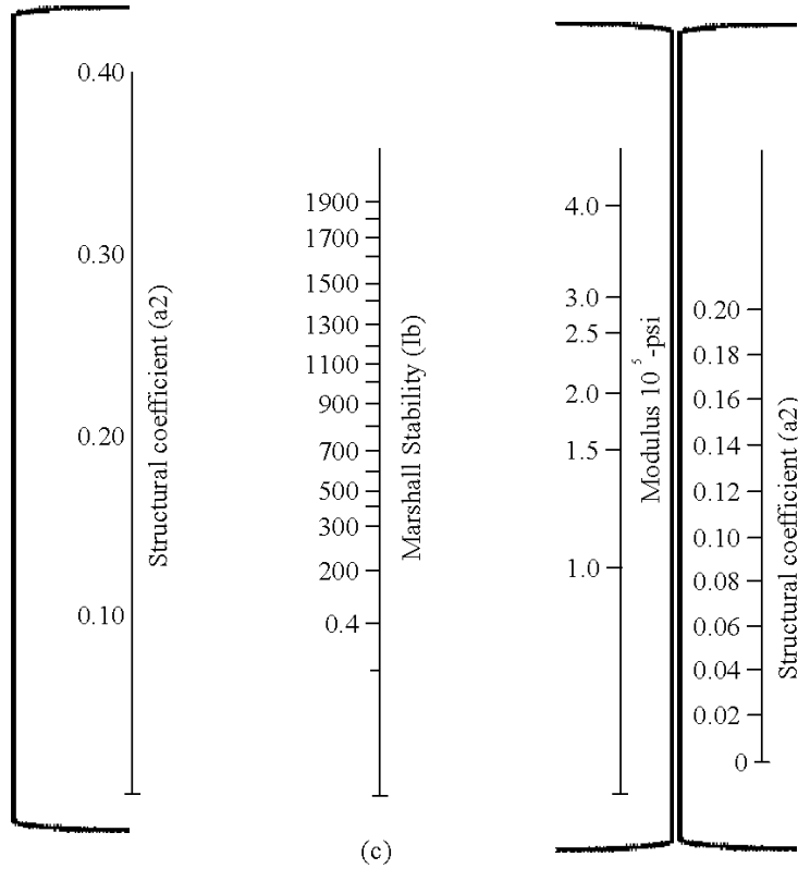
Variation in (a 2 ) for bituminous-treated bases with strength parameters
