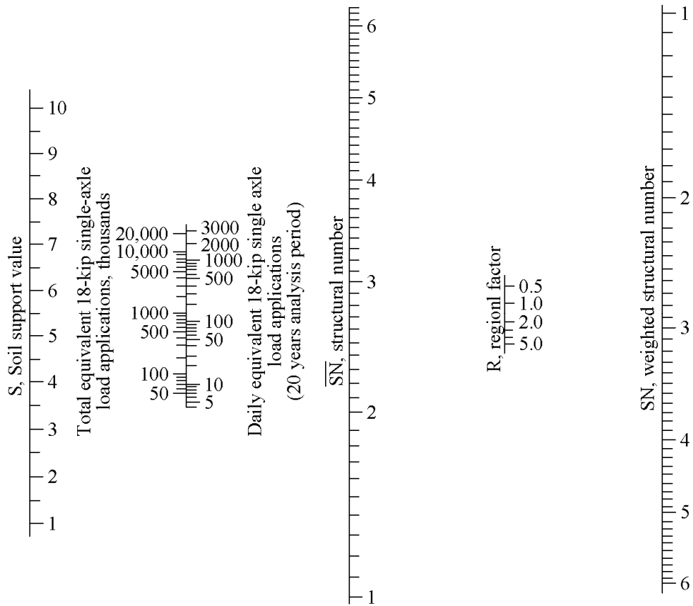
Design chart for flexible pavements, \rho_t = 2.0
