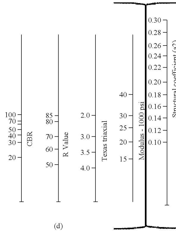
Variation in granular coefficient (a 2 ) with base strength parameters
