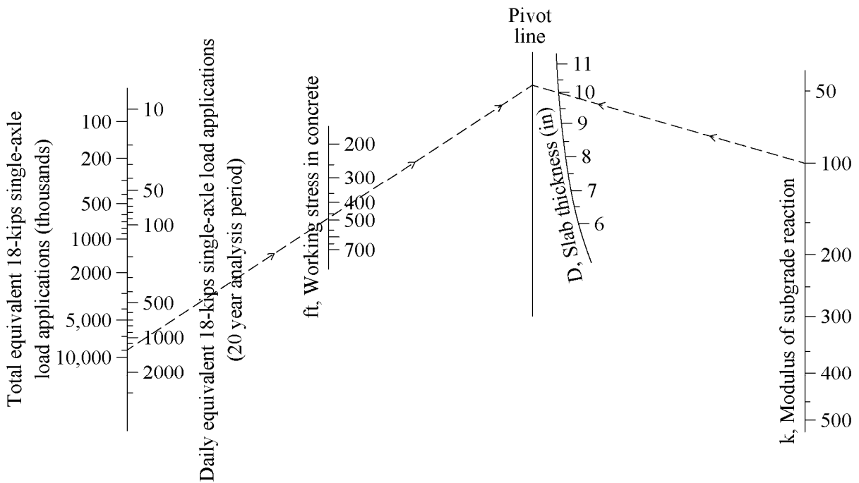
Design chart for rigid pavements, p_t = 2.5 . (From AASHO Interim Guide) Yoder, Figure 17.5, P.608
