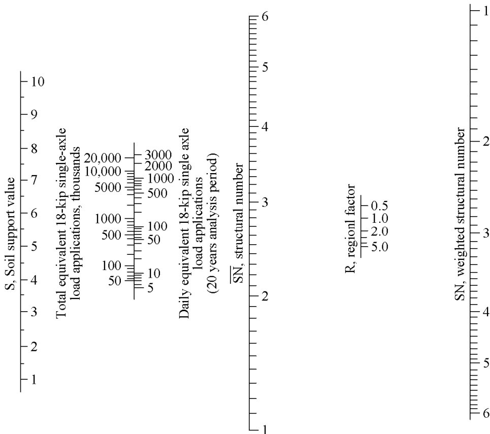
Design chart for flexible pavements, \rho_t = 2.5
