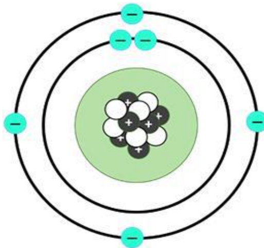
The Bohr Planetary Model
