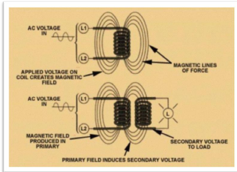
Figure 4: transformer with two windings
