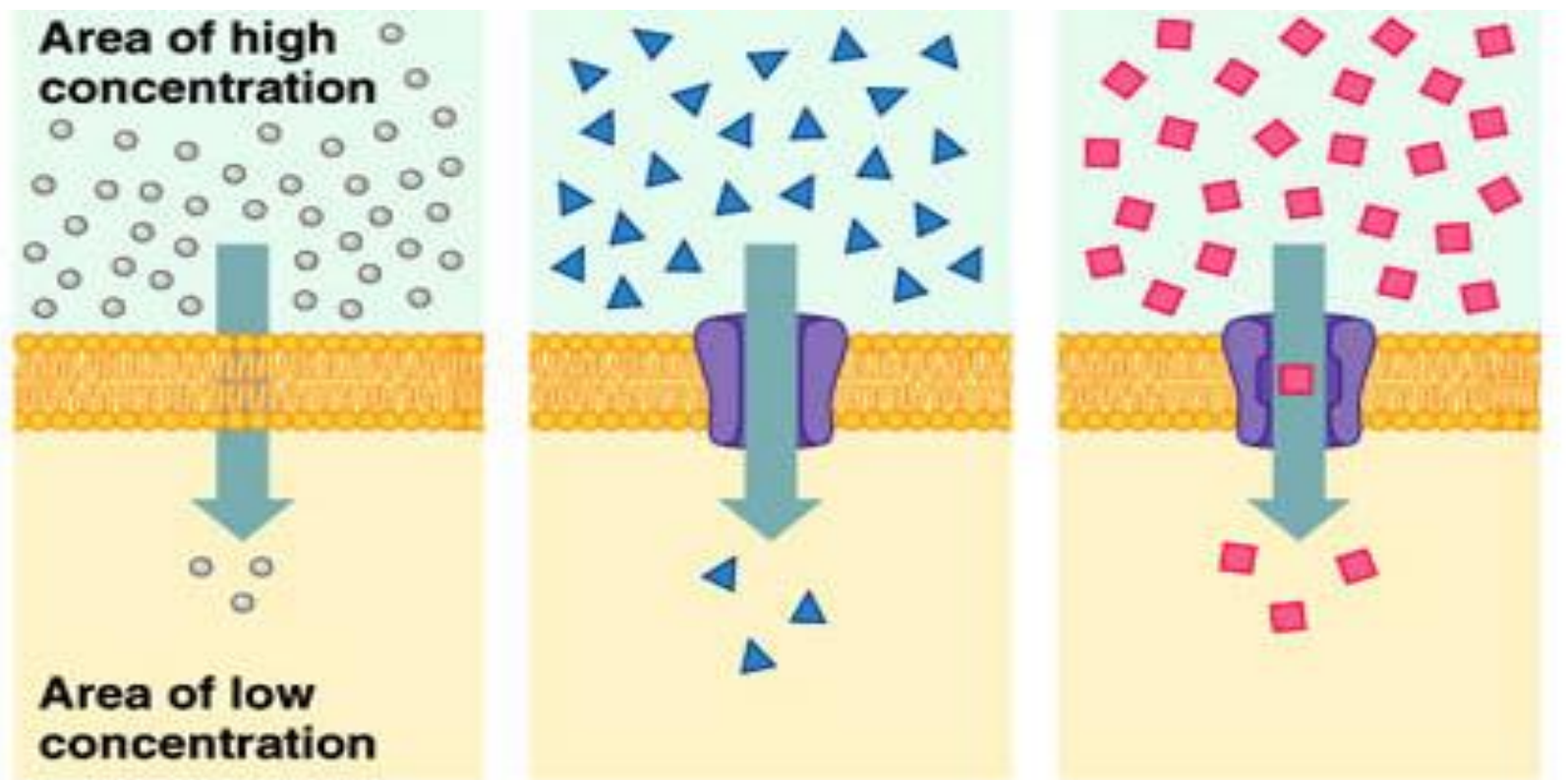
A Simple diffusion B Facilitated diffusion—channel C Facilitated diffusion—carrier
