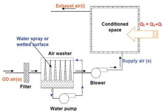
A direct, evaporative cooling system
