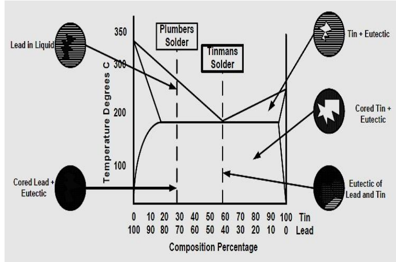
Figure 1. Lead-Tin (solder) partial solubility.
