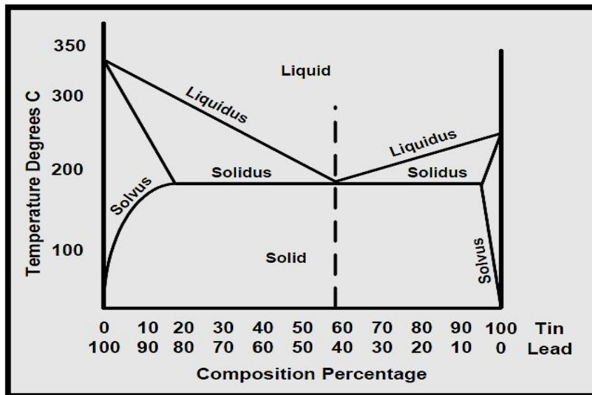
Figure 1. Lead-Tin (solder) partial solubility.
