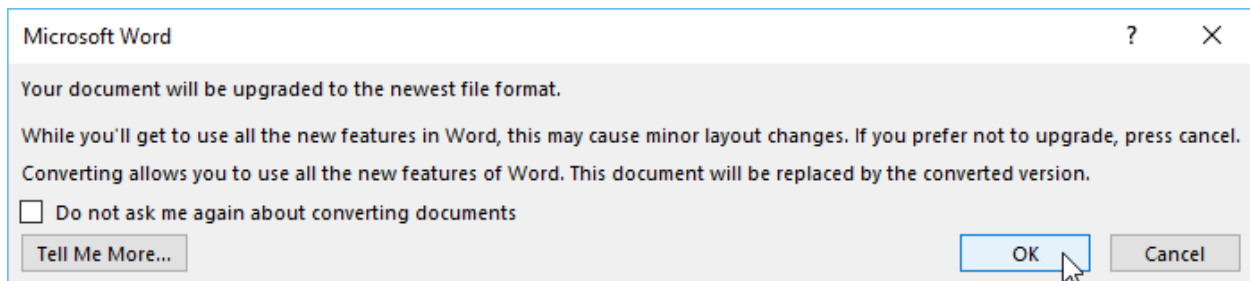
Figure 11 : convert dialog
