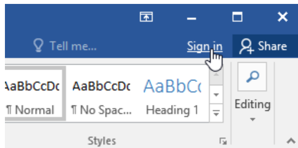
Figure 8 : onedrive signin
