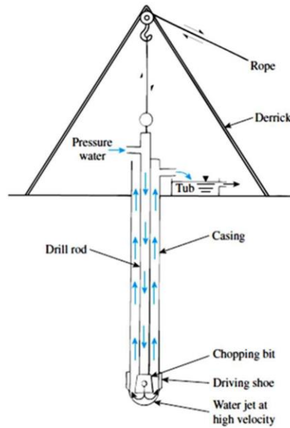
Figure 3.2 Wash boring
