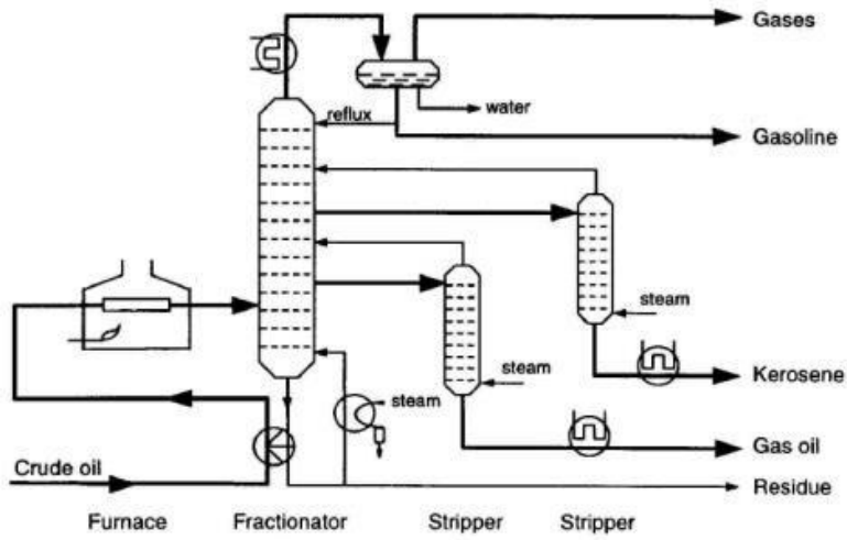
Figure 7.1: Atmospheric Distillation
