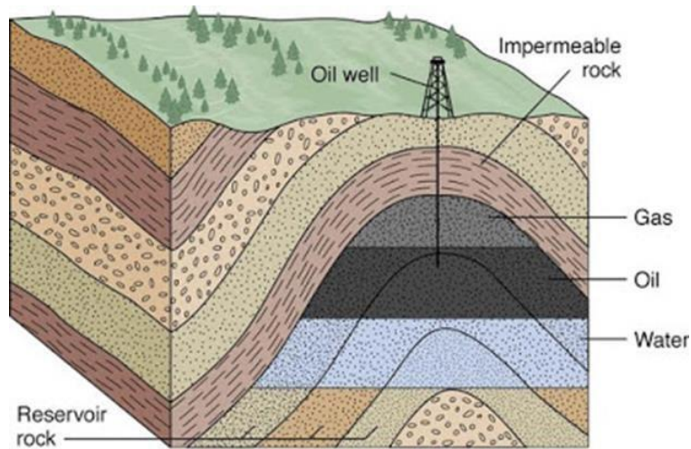
Figure 5.1. Petroleum reservoir
