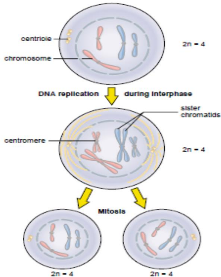
Figure 5.1 Mitosis overview.
