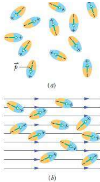
Figure 3: Molecules with a permanent electric dipole moment, showing their random orientation in the absence of an external electric field. (b) An electric field is applied, producing partial alignment of the dipoles. Thermal agitation prevents complete alignment.
