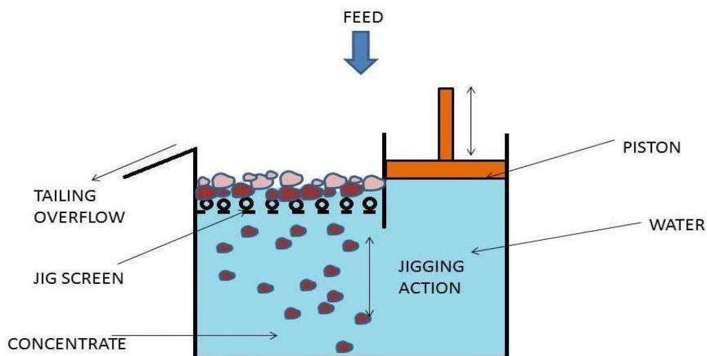
Figure 2.2 Conceptual diagram illustrates the basic principles of a jig
