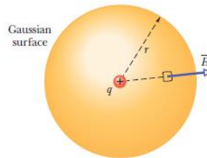
Figure 4: A spherical Gaussian surface centered on a particle with charge q .
