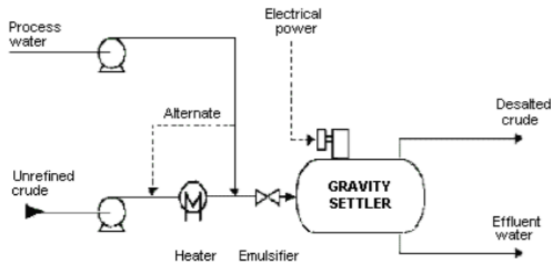
Figure 4.4- Electrical desalting
