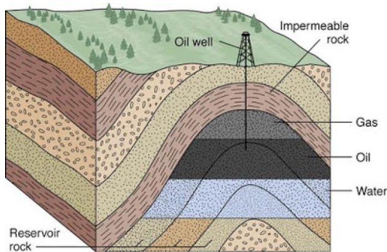
Figure 5.1. Petroleum reservoir
