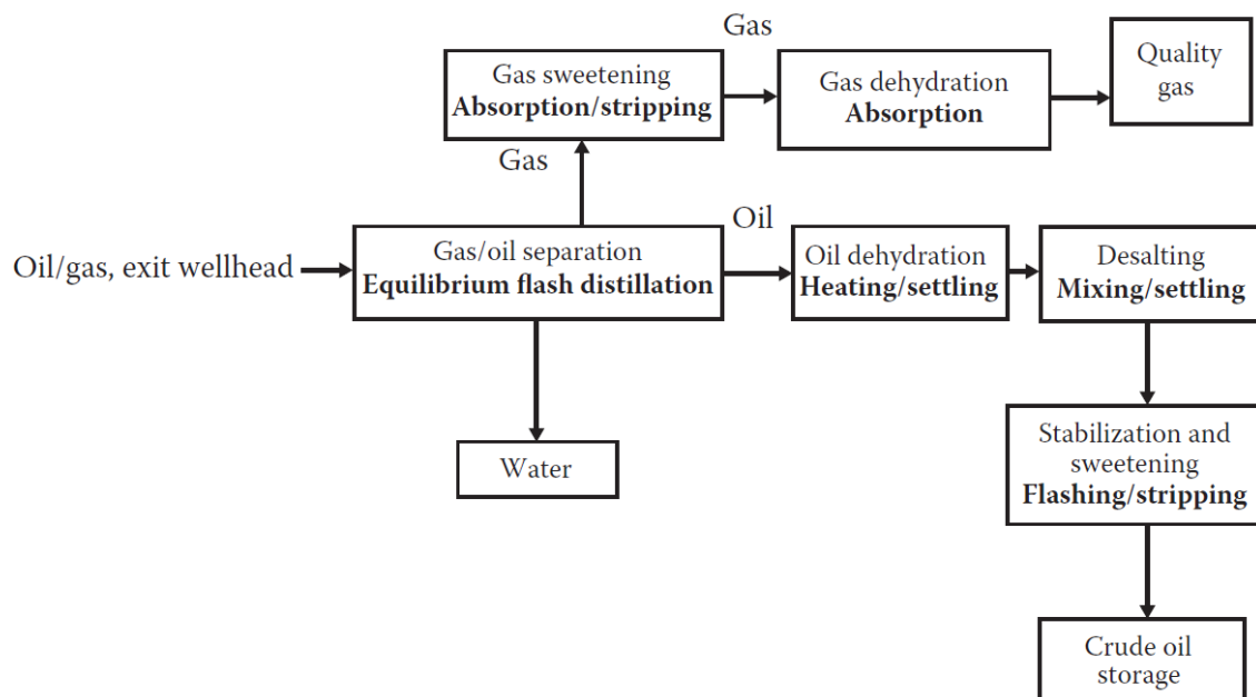
Figure 5.2. Pre-treatment unit of crude oil and gas.
