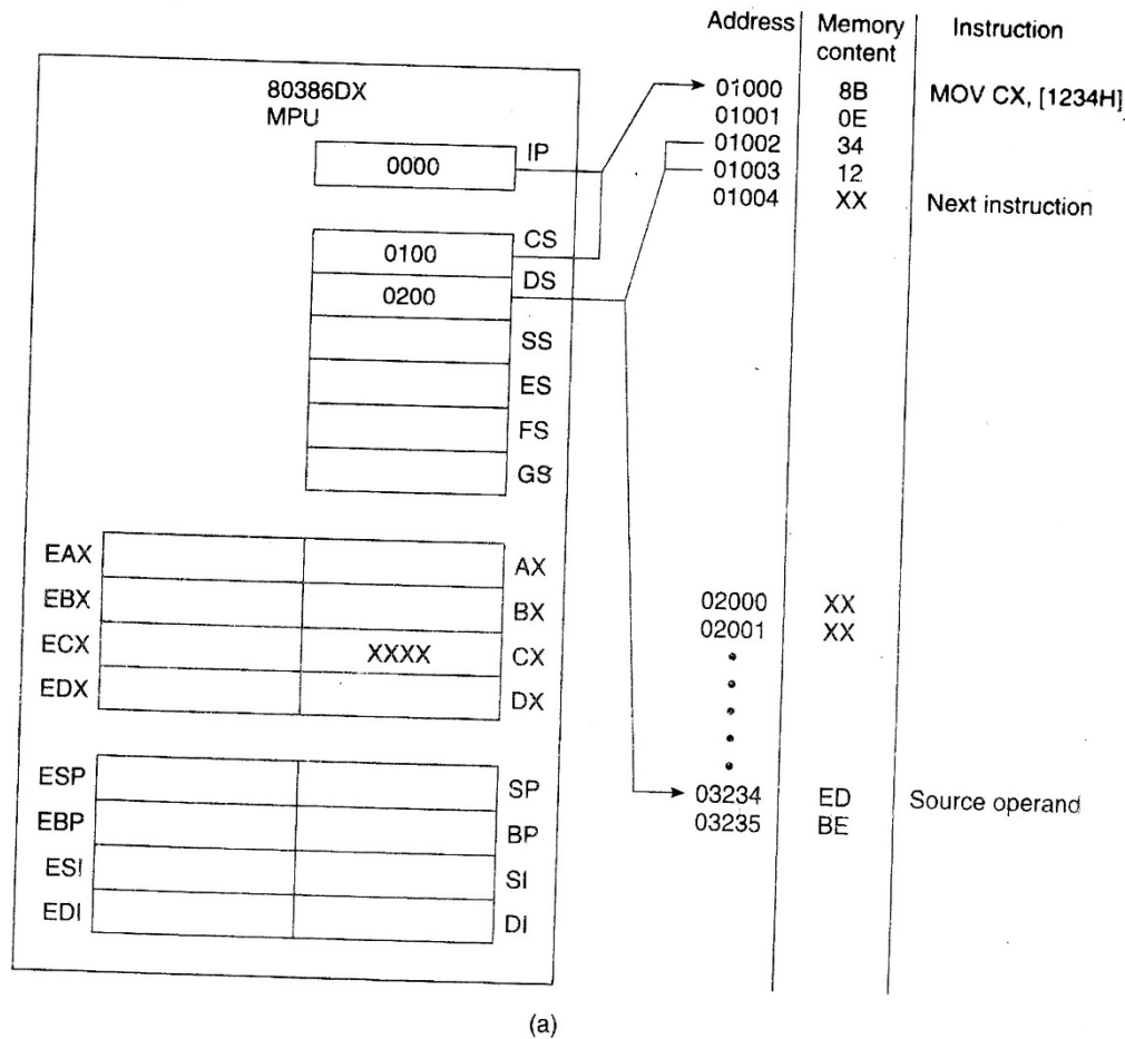
Figure 3.13 (a) Direct addressing mode instruction before fetch and execution. (b) After execution.
