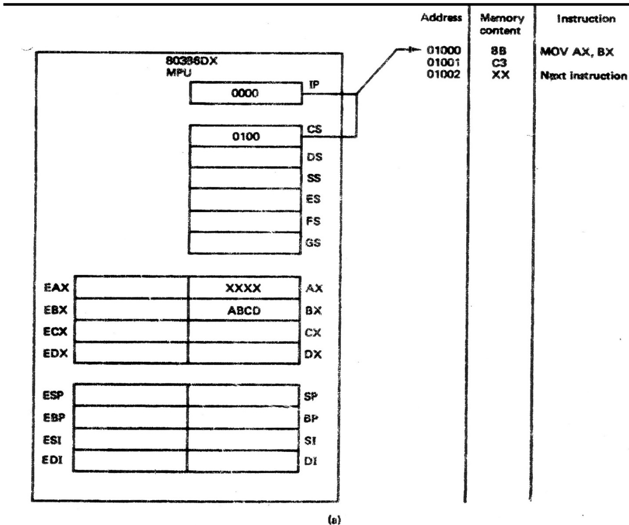
Figure 3.8 (a) Register addressing mode instruction before fetch and execution. (b) After execution.
