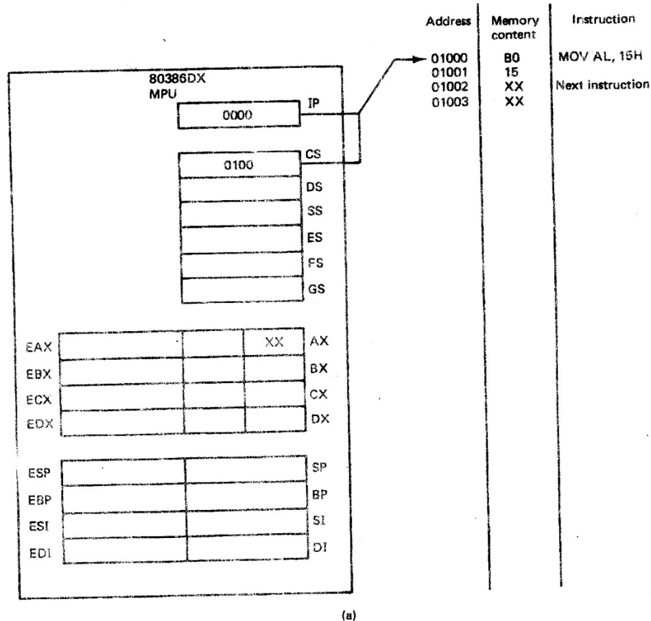
Figure 3.10 (a) Immediate addressing mode instruction before fetch and execution. (b) After execution.
