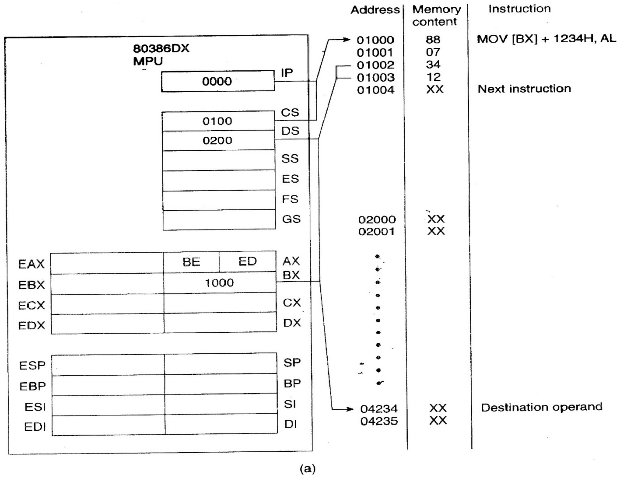
Figure 3.17 (a) Instruction using direct base pointer addressing mode before fetch and execution. (b) After execution.
