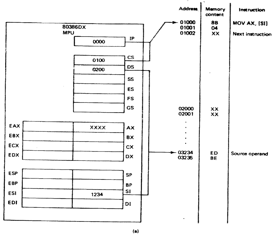
Figure 3.15 (a) Instruction using register indirect addressing mode before fetch and execution. (b) After execution.
