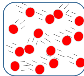
Non-Ideal Gas
