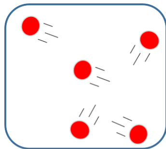
Ideal Gas
